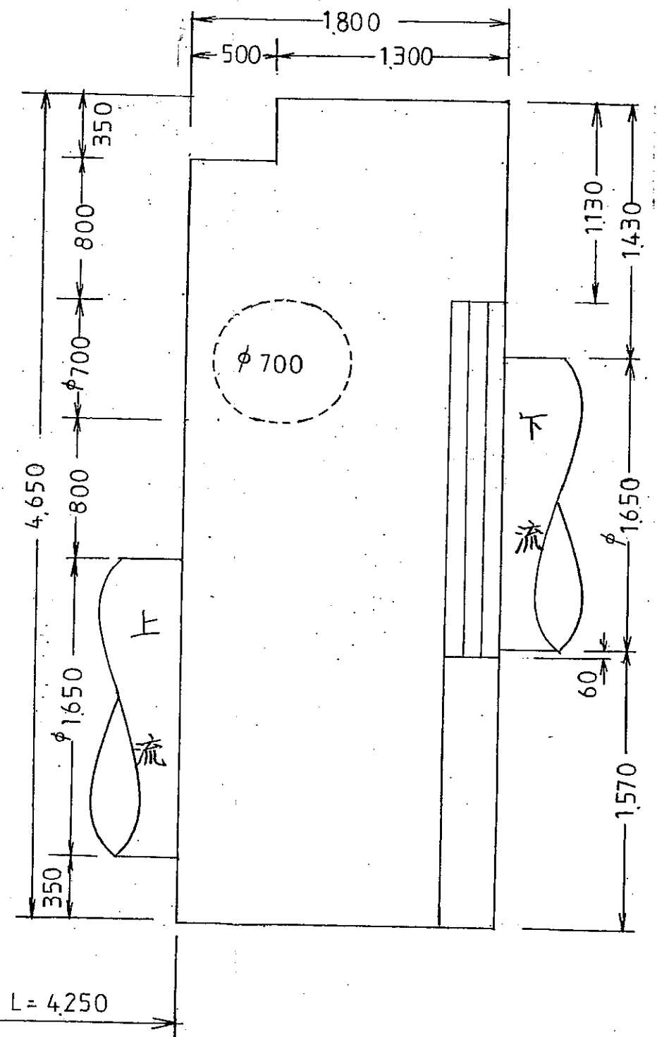
N0.2 断面図 s \frac{1}{300}
