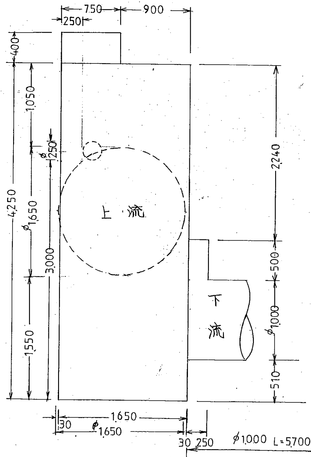
N0.1 断面図 s \frac{1}{300}
